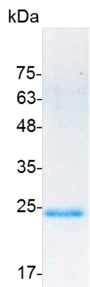
SDS-PAGE analysis of recombinant mouse 41BBL
